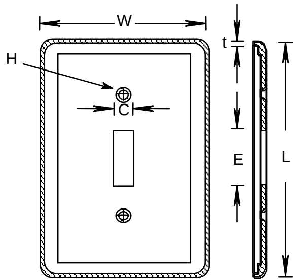
TOGGLE SWITCH, TYPE TSC15/10, 078898, 178159
