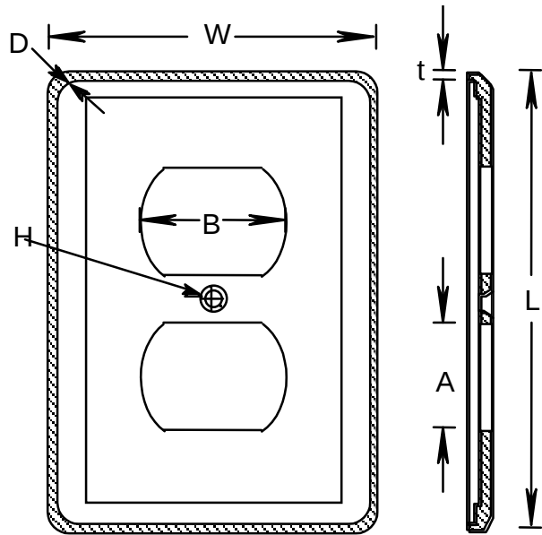
DUPLEX RECEPTACLE, TYPE DRC15/10, 078889
